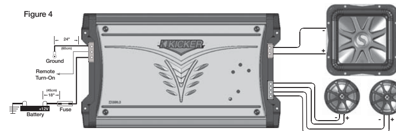
(ZX550.3) Two Channel Operation with Subwoofer
